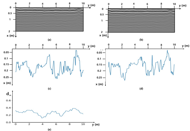
Fig. 6. Illustrations of B-scan segment from the prior map (a) and current observation (b) at a parking garage ( gates_g ) environment, and \mathbf{F}_j^{\text{shallow}} (c), \mathbf{F}_t^{\text{shallow}} (d), difference value d_m (e) between \mathbf{F}_j and \mathbf{F}_t when \mathbf{P}_j in (a) is the closest to \mathbf{P}_t in (b).
