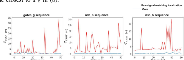
Fig. 7. e_{\text{RMSE}} over time in three environments.
