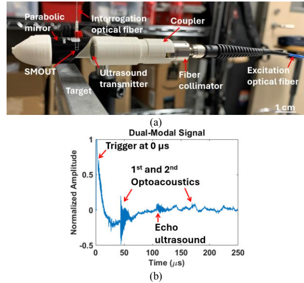
Figure 6. (a) Photograph of the prototype fabricated from the G4 sensor. (b) Representative dual-modal signal received by the G4 sensor from an aluminum block through air.
