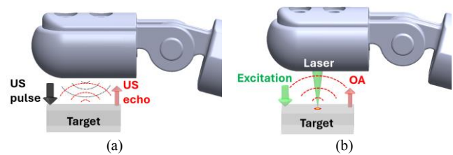
Figure 1. Illustration of the PDM 2 mechanisms: (a) pulse-echo ultrasound (US), (b) pulsed laser, and induced optoacoustics (OA).
